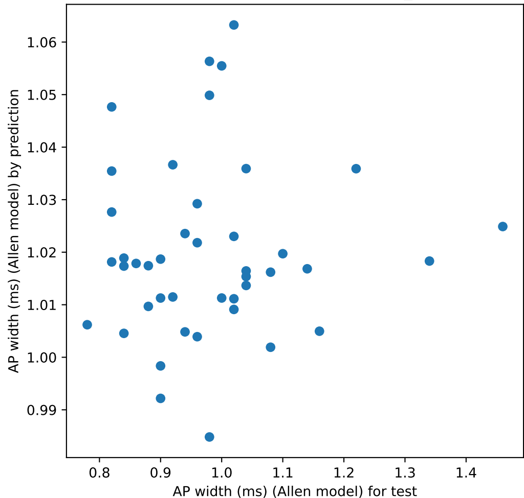
prediction of AP width (ms) (Allen model) by pcs alpha 0.25 l1_ratio 0.05 positive True MAE 0.111
